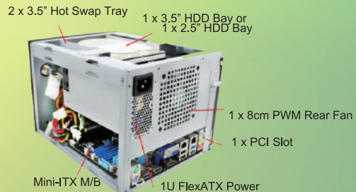
2x3.5" Hot-Swap
